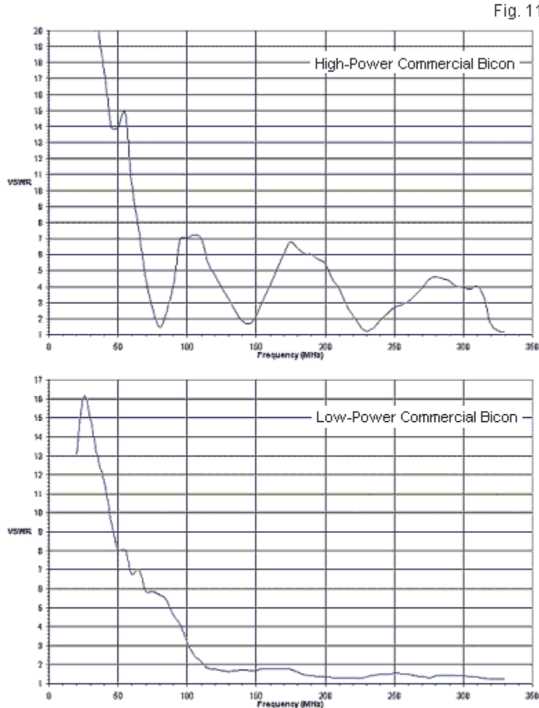
Typical Commercial Biconical Antenna SWR Curves
